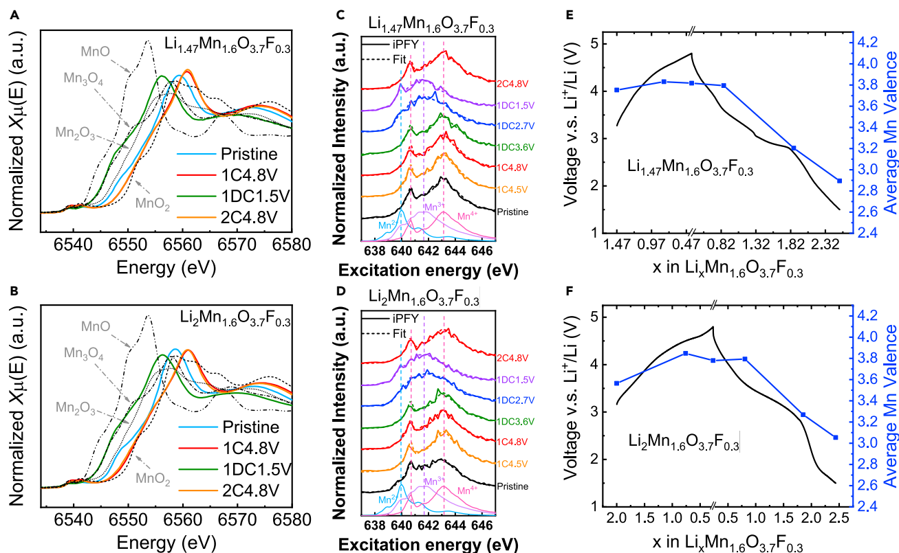
Figure 8. Redox mechanism of \text{Li}_{1.47}\text{Mn}_{1.6}\text{O}_{3.7}\text{F}_{0.3} and \text{Li}_2\text{Mn}_{1.6}\text{O}_{3.7}\text{F}_{0.3}
