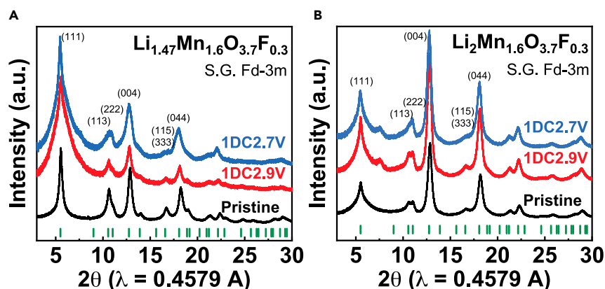
Figure 10. Ex situ synchrotron XRD of cycled cathode samples
