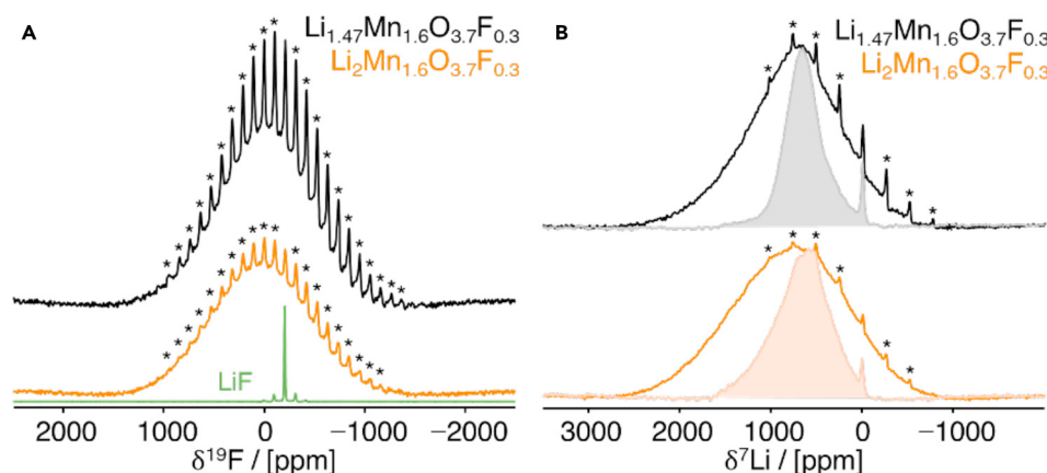
Figure 4. ssNMR spectra obtained on the as-synthesized partially (dis)ordered spinel materials
