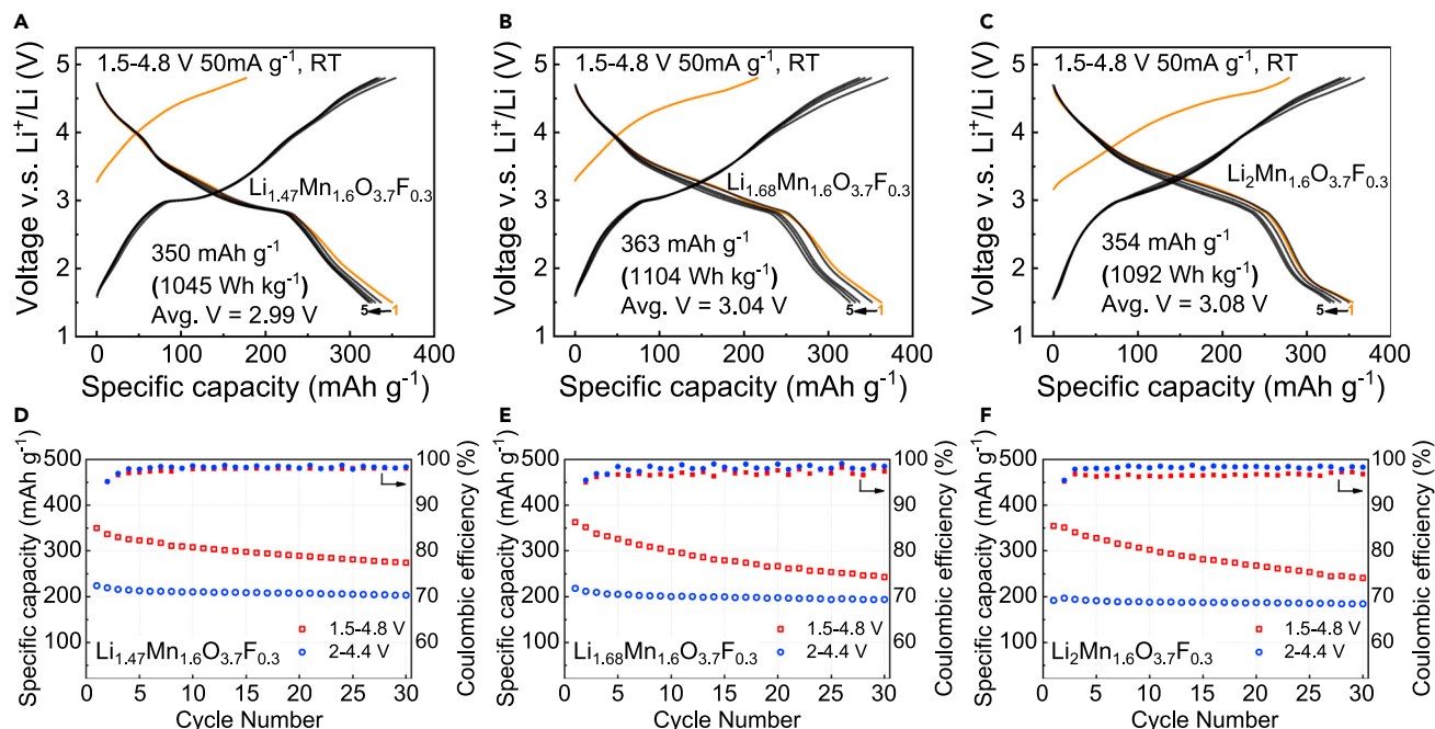
Figure 6. Galvanostatic cycling performance
