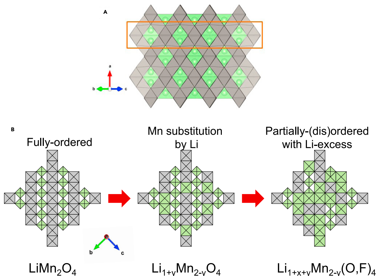
Figure 1. Design of partially (dis)ordered spinel cathodes with Li over-stoichiometry x and Mn substitution by Li y
