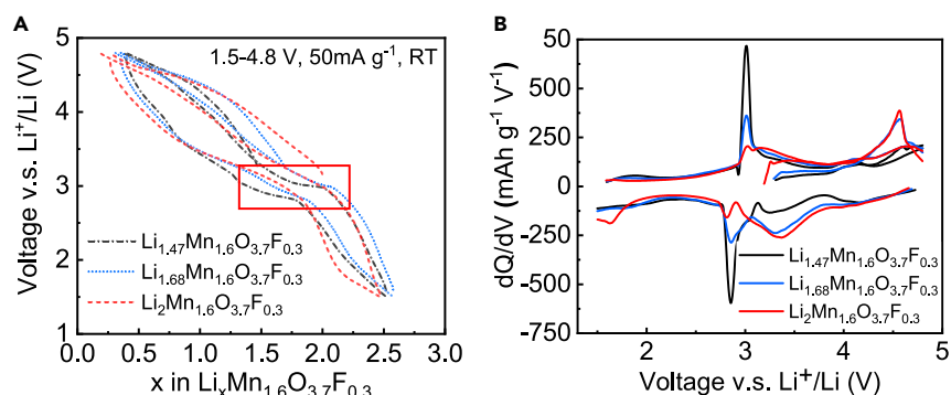
Figure 5. Galvanostatic charge and discharge performance
