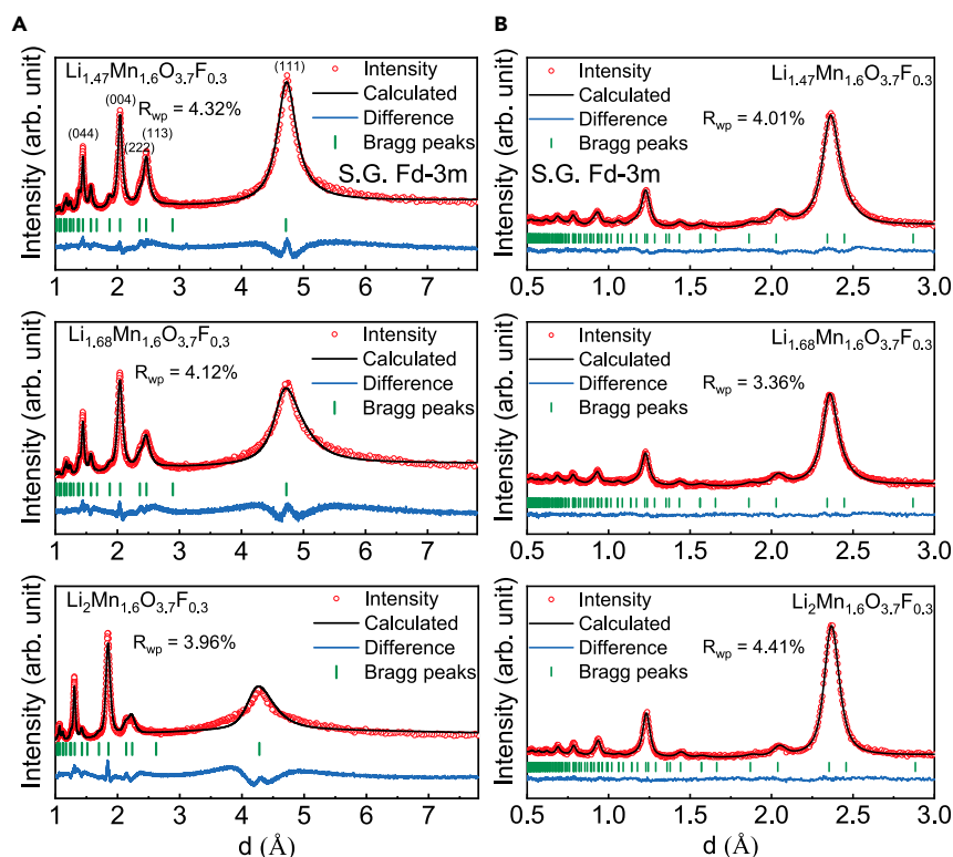
Figure 2. Refinement of three partially (dis)ordered spinels
